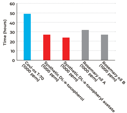
Oxidative Stability Index (OSI) in sunflower oil at 110°C
